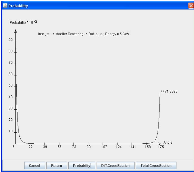
Fig. 15. Probability |M|^2 for Moeller Scattering
