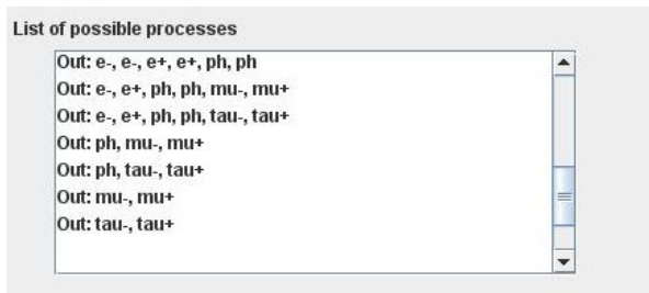
Fig. 7. List of processes including tauon pair creation
