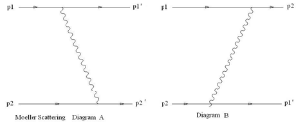
Fig. 14. Diagrams for Moeller Scattering
