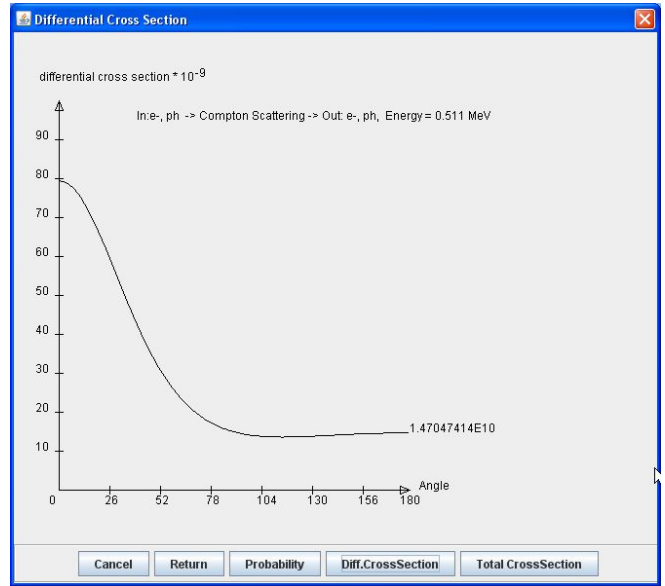
Fig. 13. Differential Cross Section for Compton Scattering
