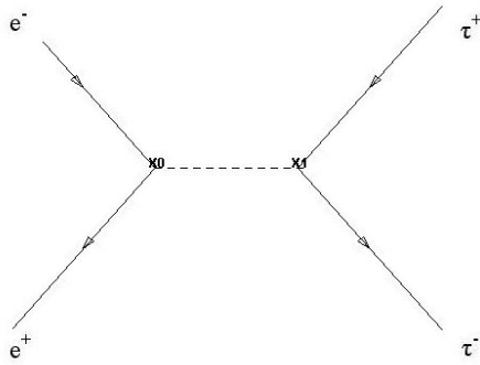
Fig. 10. Diagram for tauon pair creation including Z0 interaction
