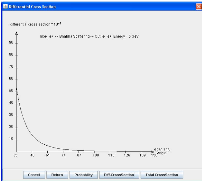
Fig. 6. Result of "Eval.Ampl." for Bhabha scattering
