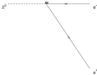
Fig. 16. Diagram for Z0-Decay
