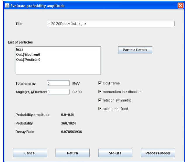
Fig. 17. Evaluation of |M|^2 and Decay Rate for Z0-Decay
