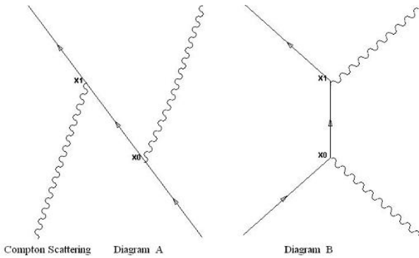
Fig. 12. Diagrams of Compton scattering
