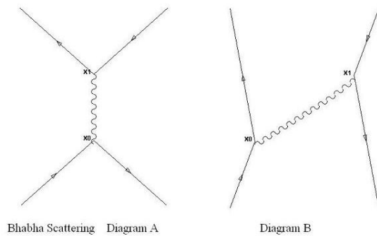
Fig. 3. Two Feynman Diagrams for Bhabha Scattering
